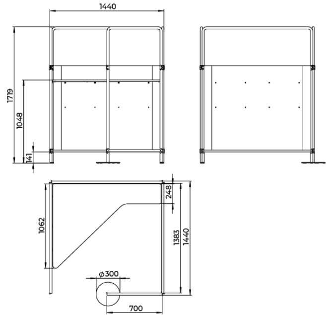
FourPeople - Work booth setup - H1720 - W1400xW1400xW1400xW700 - with tabletop
